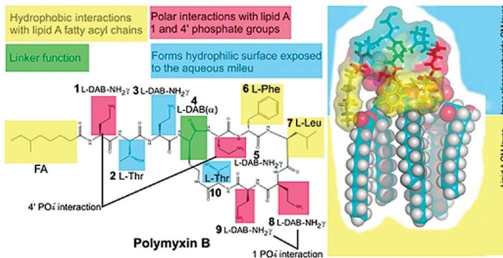
Figure 4. A color coded schematic diagram summarizing the key contacts involved in complex formation between PMB and the lipid A component of LPS. FA = N -terminal fatty acyl chain.
