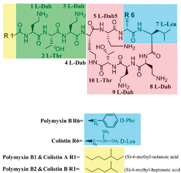
Figure 1. Chemical structures of polymyxin B and colistin. The functional segments of polymyxins are colored as follows: yellow, N^{\alpha} fatty acyl chain; green, linear tripeptide segment; red, the polar residues of the heptapeptide; blue, the hydrophobic motif within the heptapeptide ring. The amino acids positions are numbered in accordance to references in the text.
